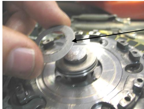
Needle Thrust Bearing
